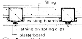
① Acoustic improvement with suspended ceiling
